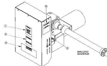
POWER-TAKE-OFF DRIVE
